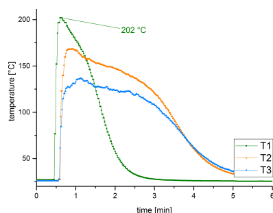
Figure 1: Temperature profile for the reaction of \text{NH}_3 with \text{CuSO}_4 on zeolithe
